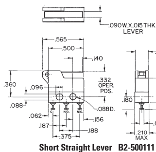
Short Straight Lever B2-500111
