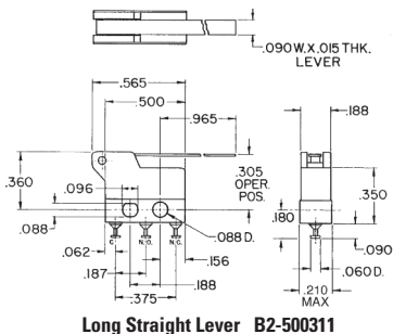
Long Straight Lever B2-500311
