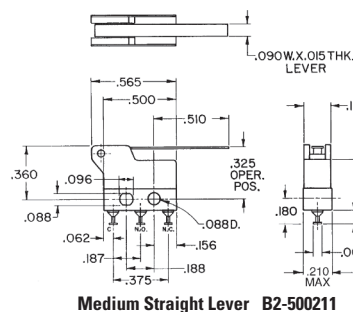
Medium Straight Lever B2-500211
