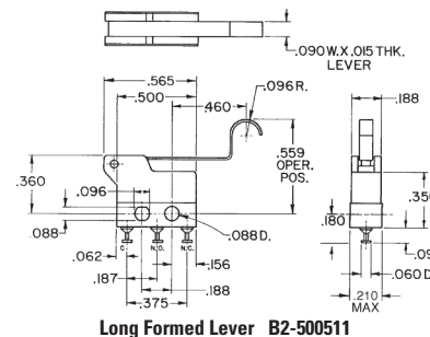
Long Formed Lever B2-500511
