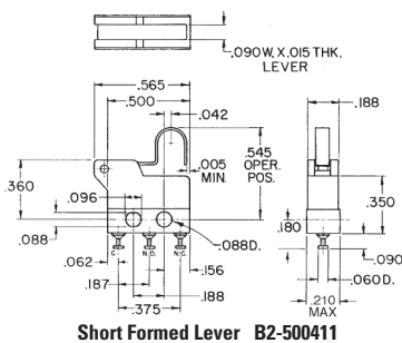
Short Formed Lever B2-500411
