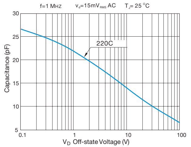
Typical Capacitance vs. Off-state Voltage
