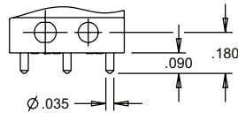
TERMINAL STYLE 2 DOUBLE SOLDER TURRET
