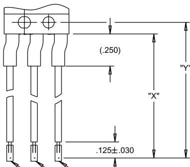
TERMINAL STYLE 5 PRINTED CIRCUIT PIN 0.270" LONG
