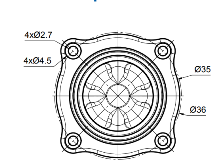
Dimensions plan view
