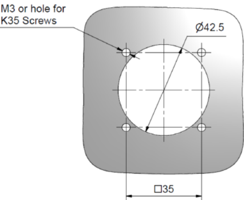
Panel cut-out
