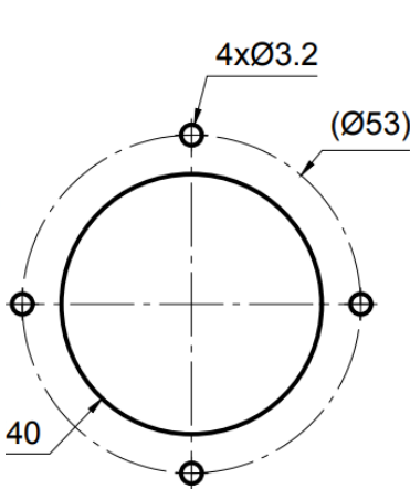
Panel cut-out
