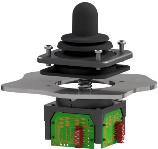
Mounting illustration with mounting ring
