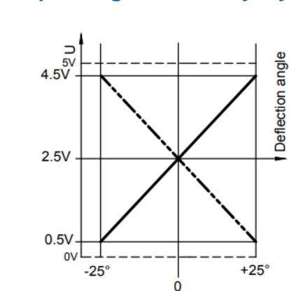
Output diagram x1, x2, y1, y2
