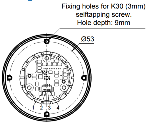
Mounting
